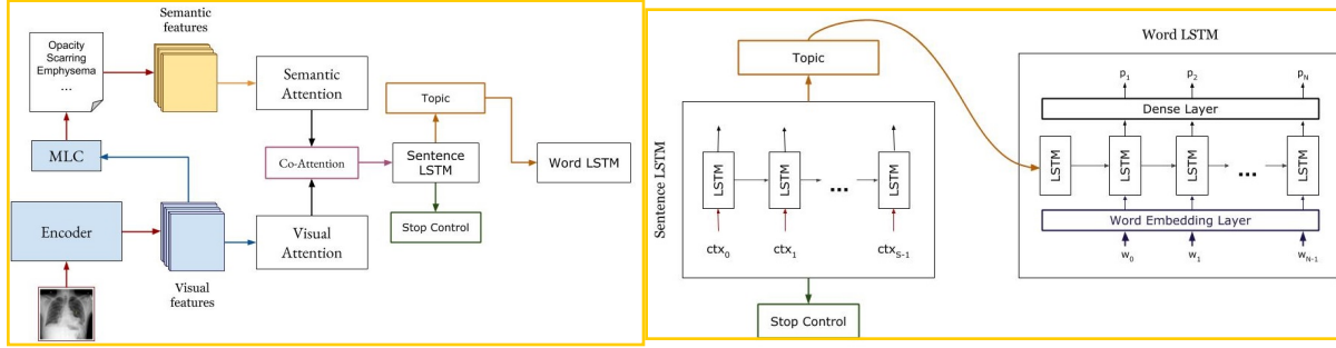
(a) Image encoder, visual and semantic features, attention mechanisms, and hierarchical decoder.
